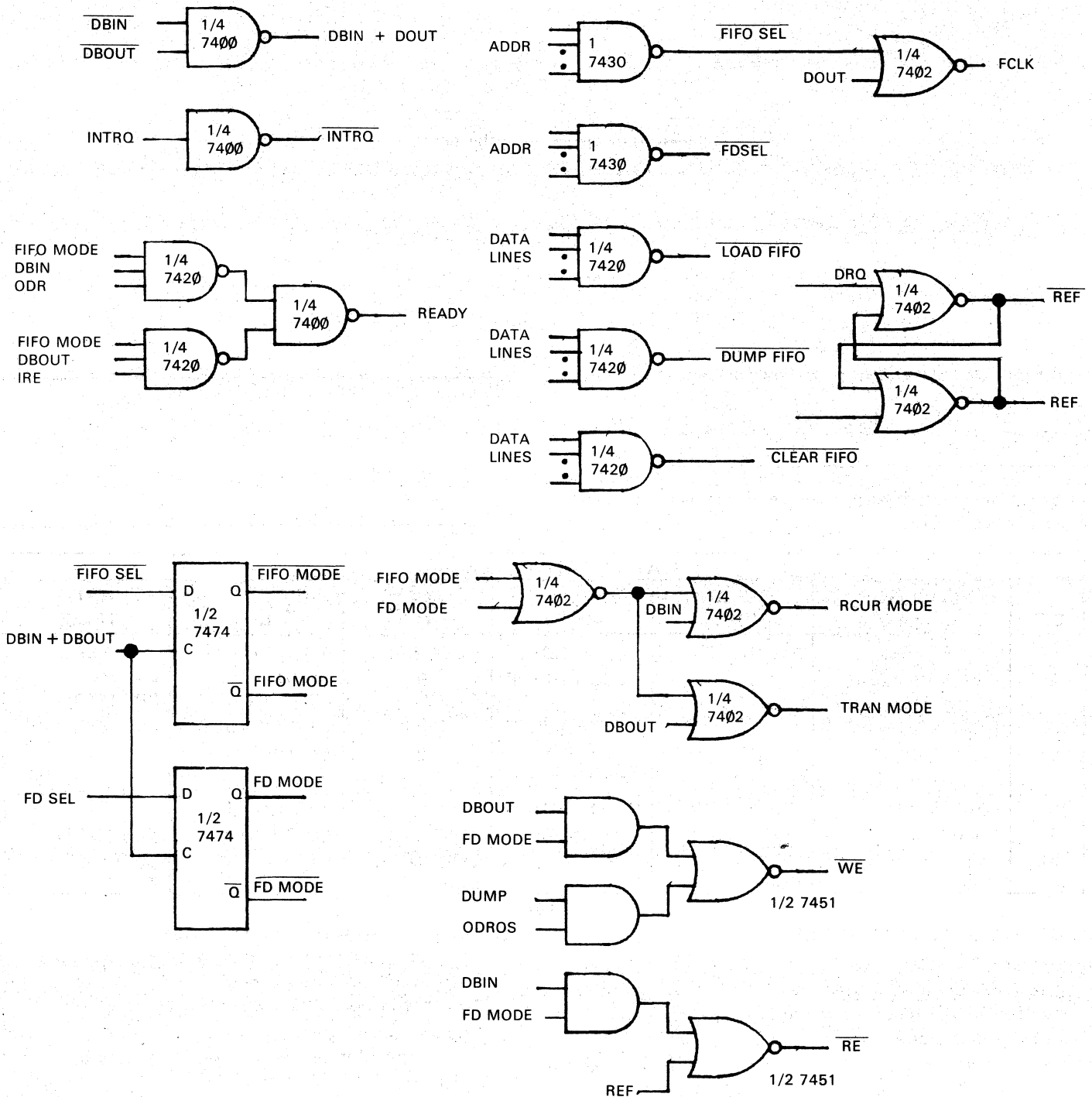
FIGURE 2-7 TIMING CONTROL
