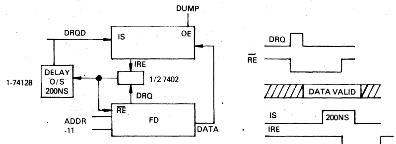
FLOPPY TO FIFO TIMING FIGURE 2-6
